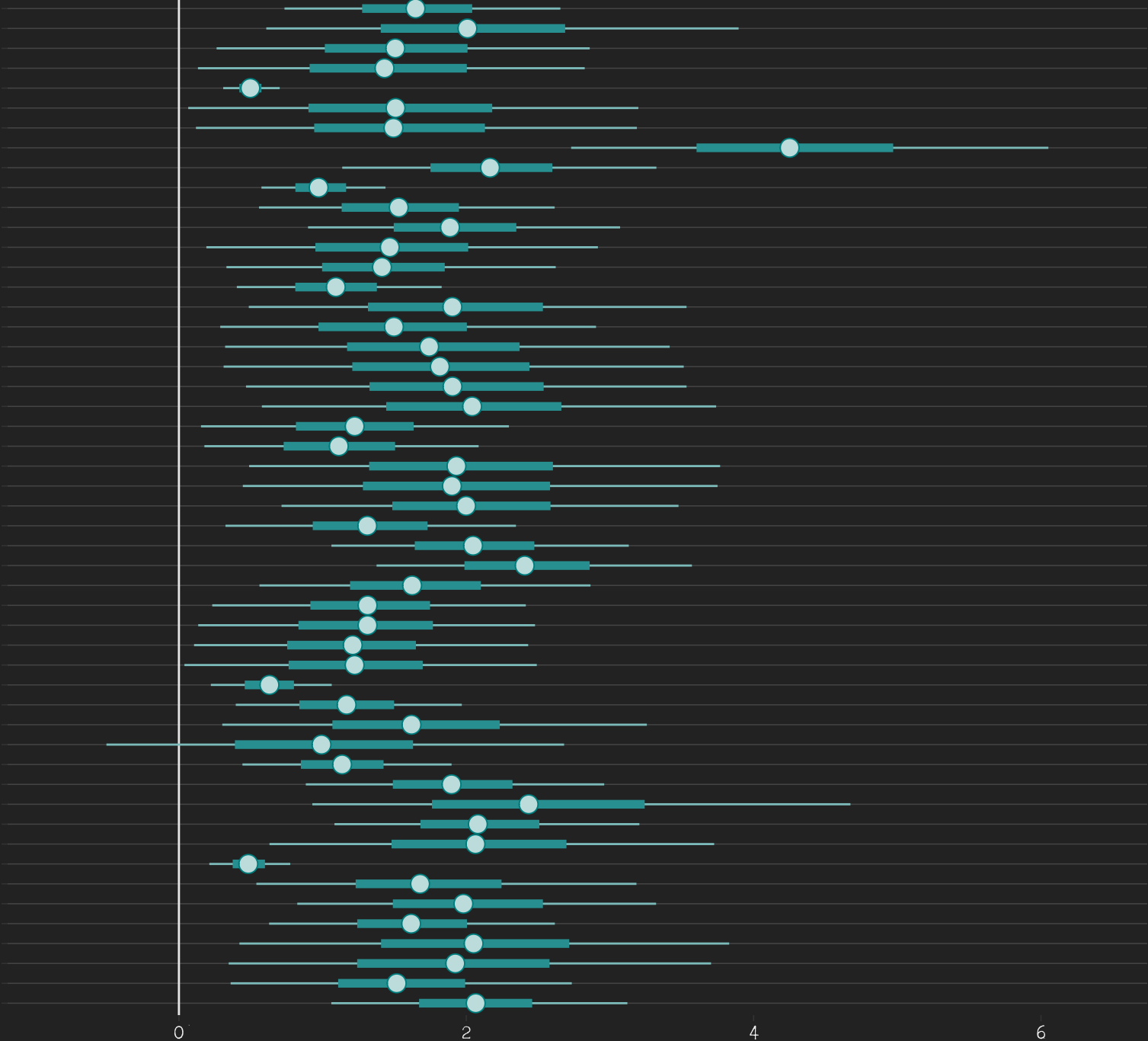
Slopes
