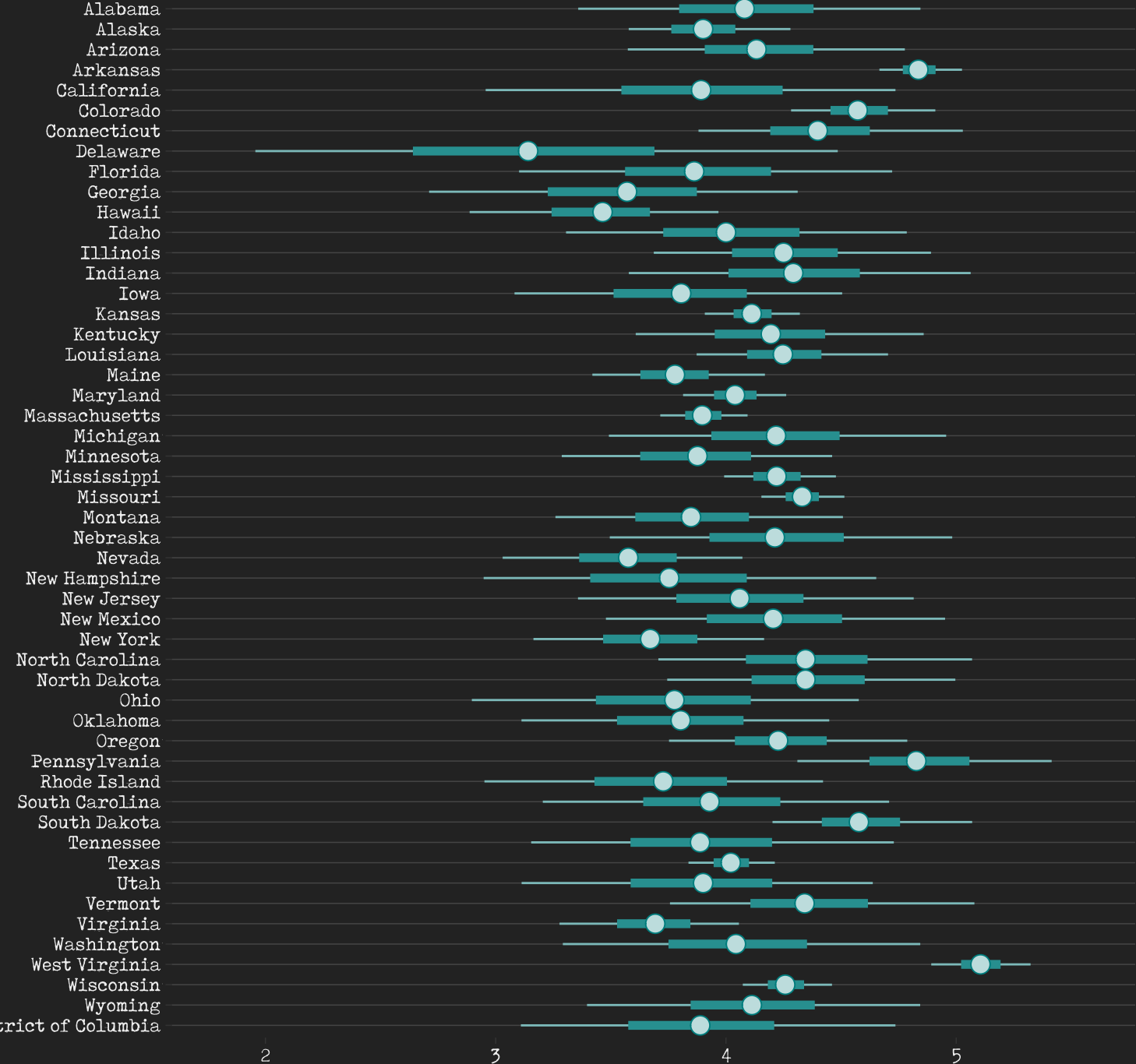
Intercepts
